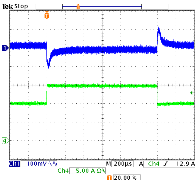
Fig.5.0V-6: Output voltage response to load current step-change (10A to 15A) at Vin=48V. Top trace: Output voltage (100mV/div). Bottom trace: load current (5A/div). Current slew rate: 5A/µs. Co=470µF os-con + 10µF tantalum + 1µF ceramic. Time scale: 200µs/div
