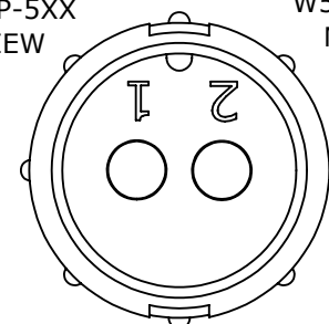
W5180-2PG-P-5XX MATING VIEW
