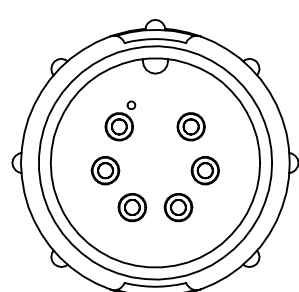
W5280-6PG-P-5XX MATING VIEW
