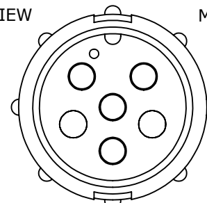
W5380-6PG-P-5XX MATING VIEW
