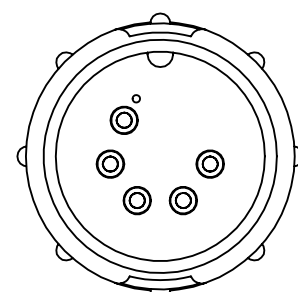
W5280-5PG-P-5XX MATING VIEW
