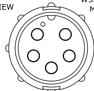
W5380-5PG-P-5XX MATING VIEW
