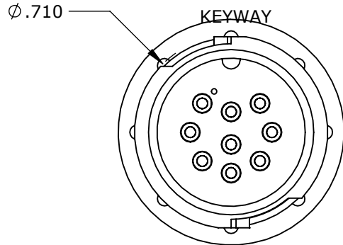
W5280-9PG-P-5XX SHOWN MATING VIEW
