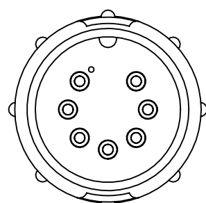
W5280-7PG-P-5XX MATING VIEW
