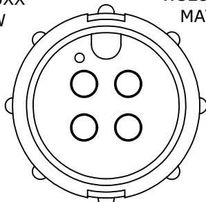
W5380-4PG-P-5XX MATING VIEW
