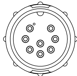
W5280-8PG-P-5XX MATING VIEW
