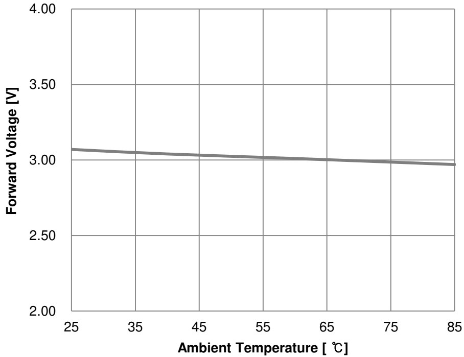
Fig 7. Ambient Temperature vs. Forward Voltage, I_F=100mA
