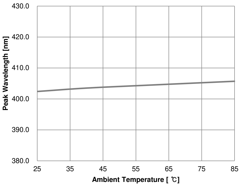
Fig 6. Ambient Temperature vs. Peak Wavelength, I_F=100mA
