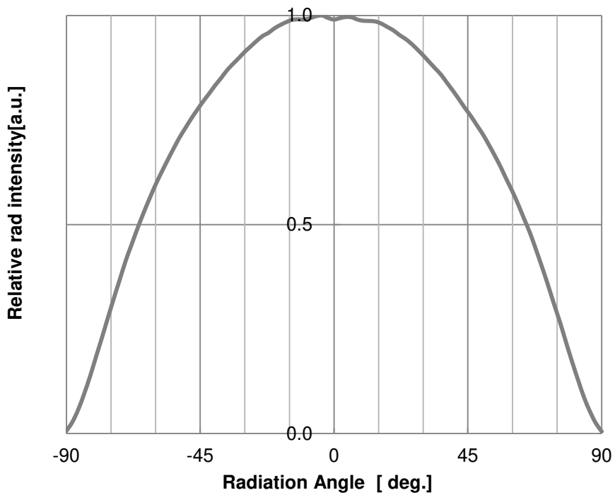
Fig 8. Typical Spatial Distribution, I_F=100mA
