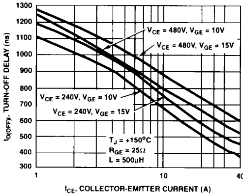
FIGURE 9. TURN-OFF DELAY vs COLLECTOR-EMITTER CURRENT
