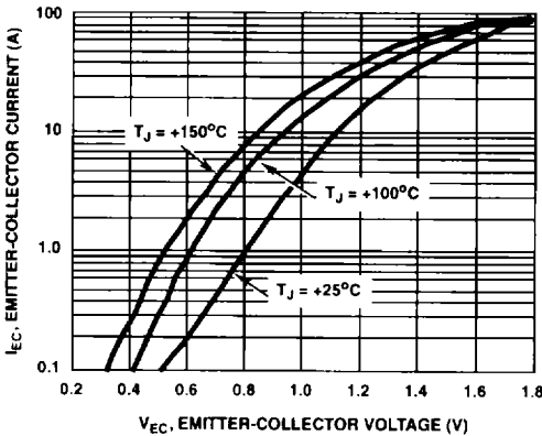
FIGURE 11. FORWARD VOLTAGE vs FORWARD CURRENT CHARACTERISTIC
