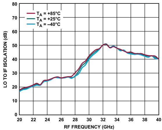
Figure 86. LO to IF Isolation vs. RF Frequency at Various Temperatures, LO = 13 dBm
