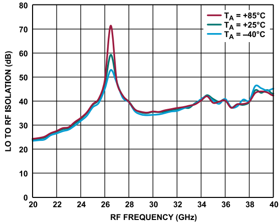
Figure 85. LO to RF Isolation vs. RF Frequency at Various Temperatures, LO = 13 dBm
