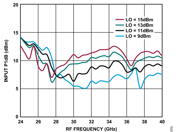
Figure 66. Input P1dB vs. RF Frequency at Various LO Power Levels, T_A = 25^\circ\text{C}
