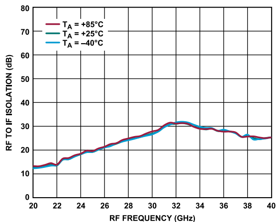
Figure 87. RF to IF Isolation vs. RF Frequency at Various Temperatures, LO = 13 dBm
