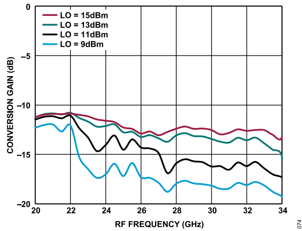
Figure 70. Conversion Gain vs. RF Frequency at Various LO Power Levels, T_A = 25^\circ\text{C}
