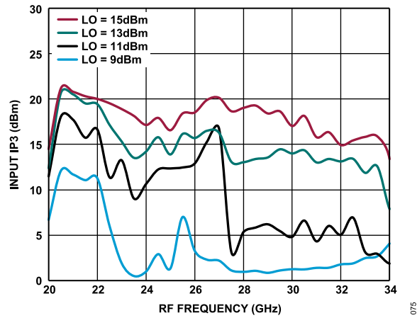
Figure 71. Input IP3 vs. RF Frequency at Various LO Power Levels, T_A = 25^\circ\text{C}
