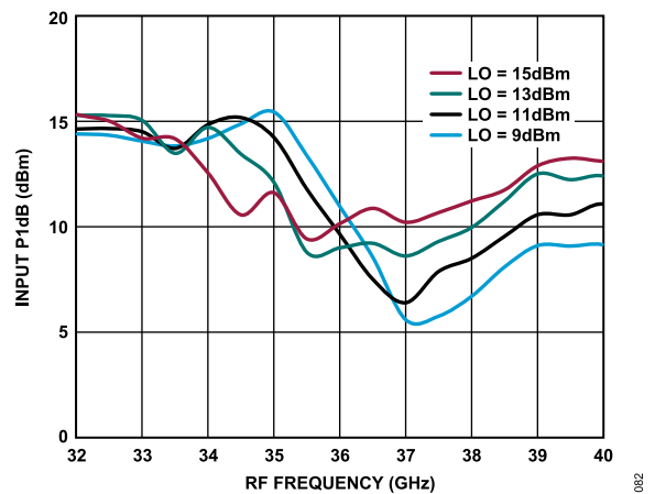
Figure 78. Input P1dB vs. RF Frequency at Various LO Power Levels, T_A = 25^\circ\text{C}
