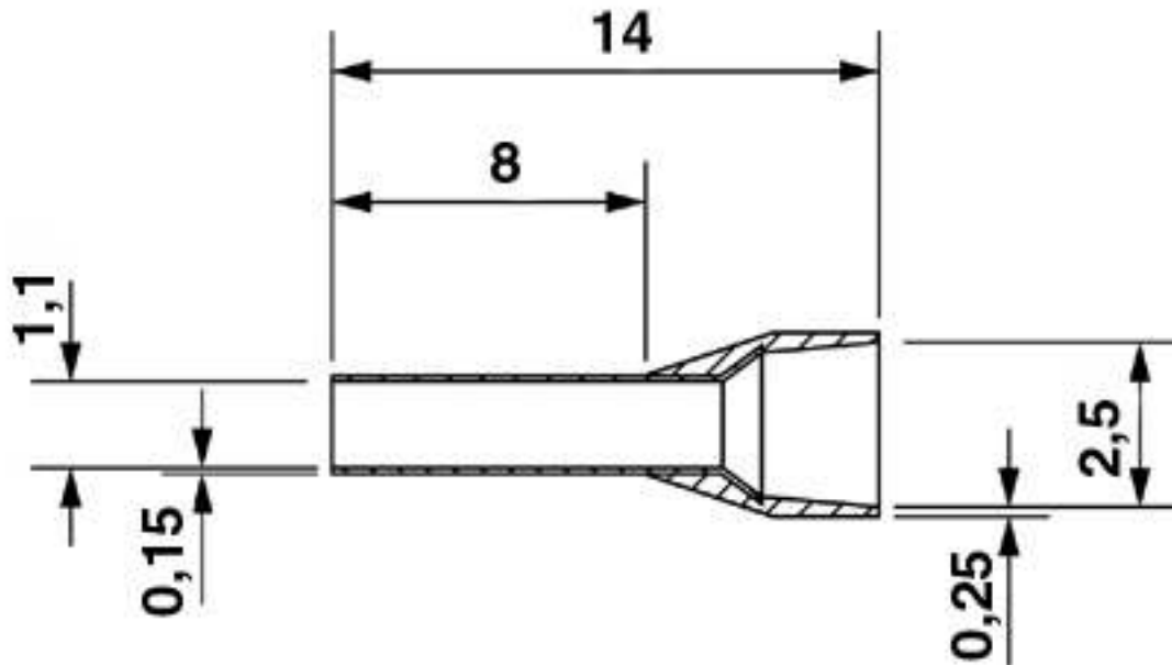
Dimensioned drawing
