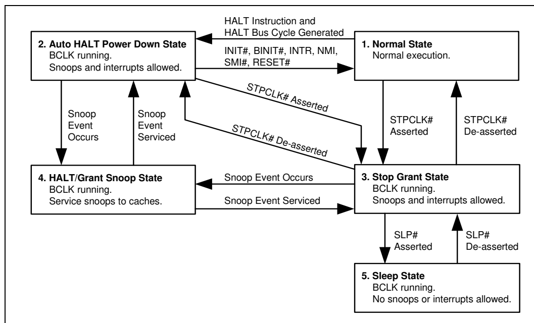
Figure 6-1. Stop Clock State Machine
