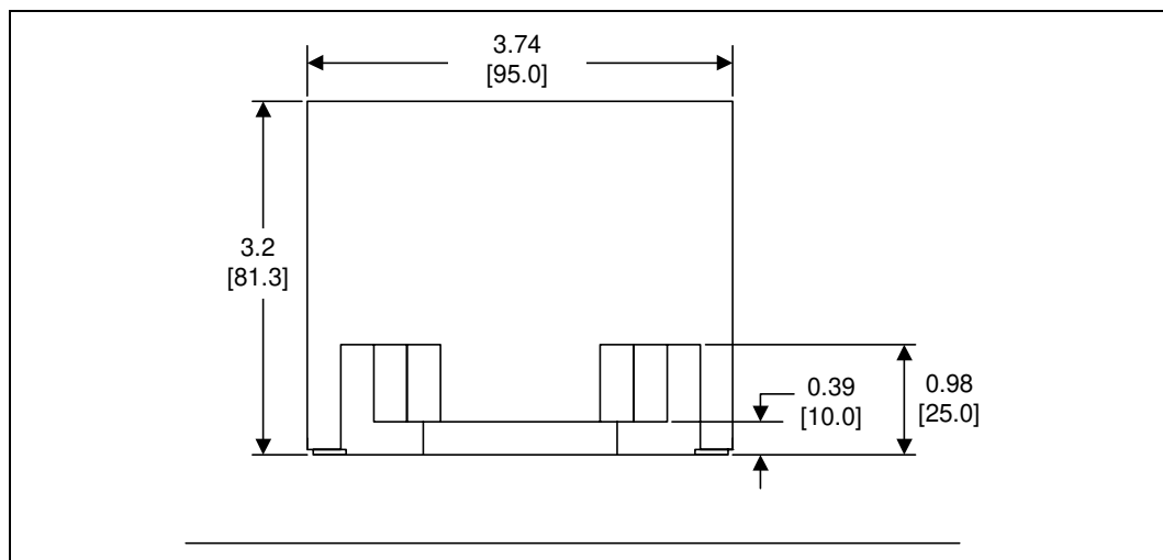
Figure 7-2. Space Requirements for the Boxed Processor (Side View)
