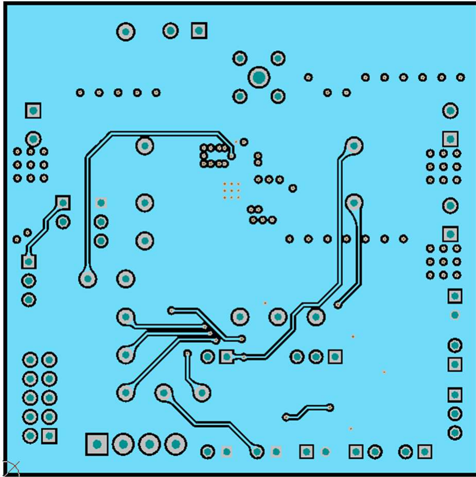
Figure 9. PWR655 EVM Third Layer
