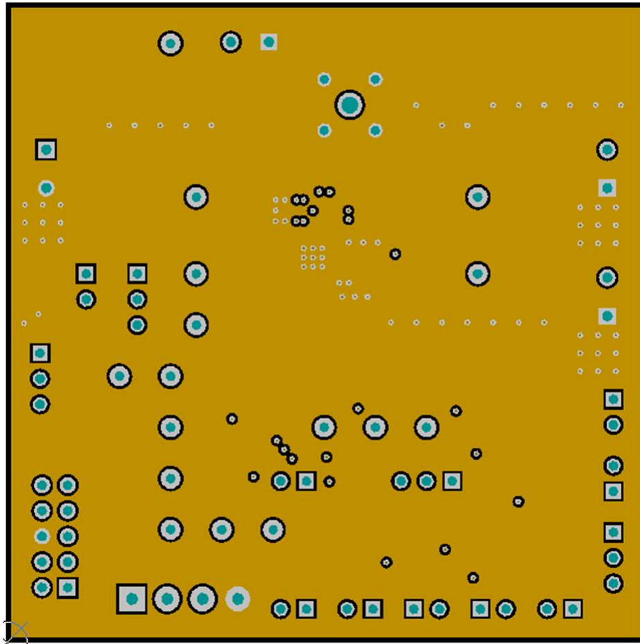
Figure 8. PWR655 EVM Second Layer
