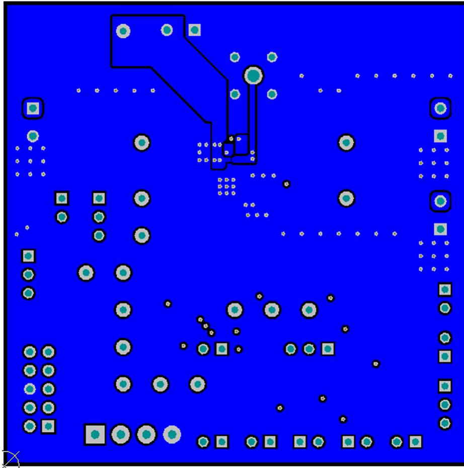
Figure 10. PWR655 EVM Bottom Layer
