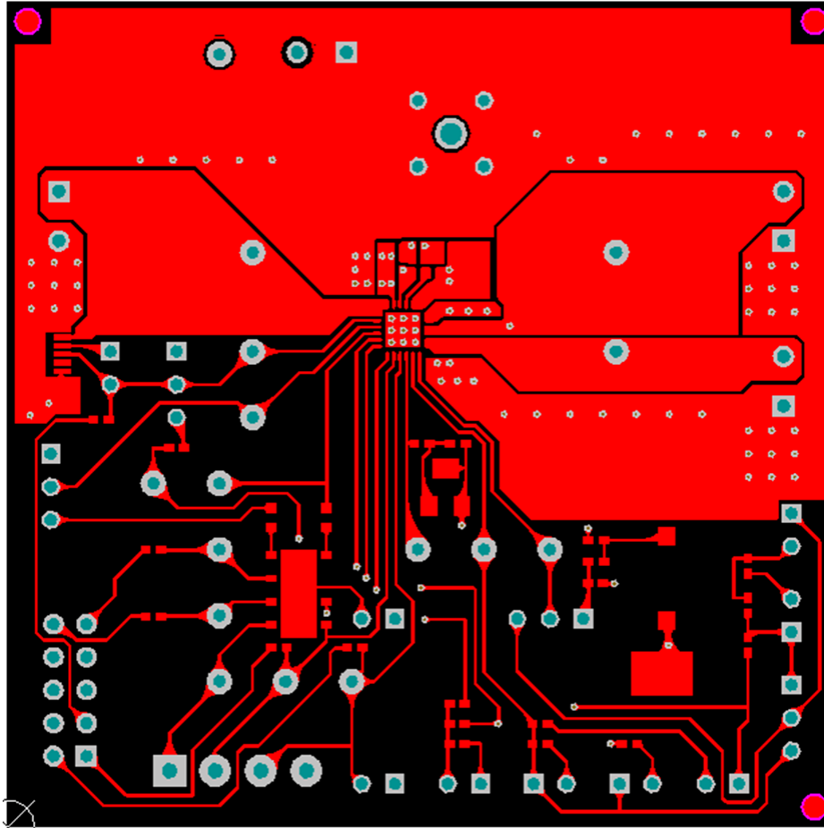
Figure 7. PWR655 EVM Top Layer
