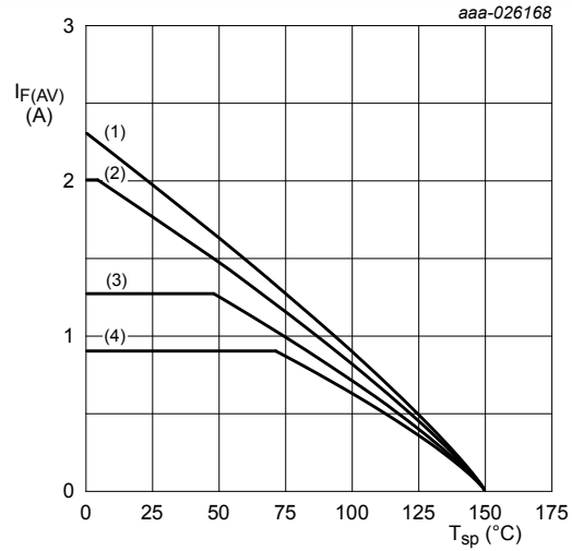
T j = 150 °C (1) δ = 1; DC (2) δ = 0.5; f = 20 kHz (3) δ = 0.2; f = 20 kHz (4) δ = 0.1; f = 20 kHz
