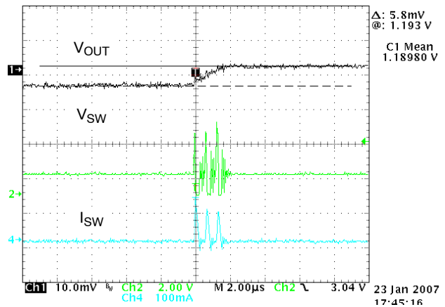
Figure 27. PFM Switching Waveforms (V_{IN} = 3.6 \text{ V}, V_{OUT} = 1.2 \text{ V}, I_{OUT} = 0 \text{ mA}, \text{Temperature} = 25^\circ\text{C})
