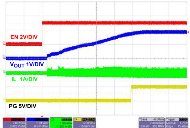
FIGURE 22. SOFT-START WITH NO LOAD (PWM)
