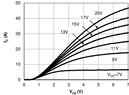
Figure 2: Output Characteristic ( T_j=150^\circ\text{C} )
