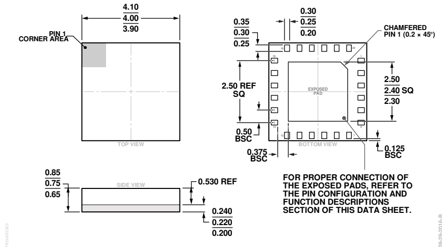
Figure 44. 24-Terminal Land Grid Array [LGA] 4 mm × 4 mm Body and 0.75 mm Package Height (CC-24-5) Dimensions shown in millimeters
