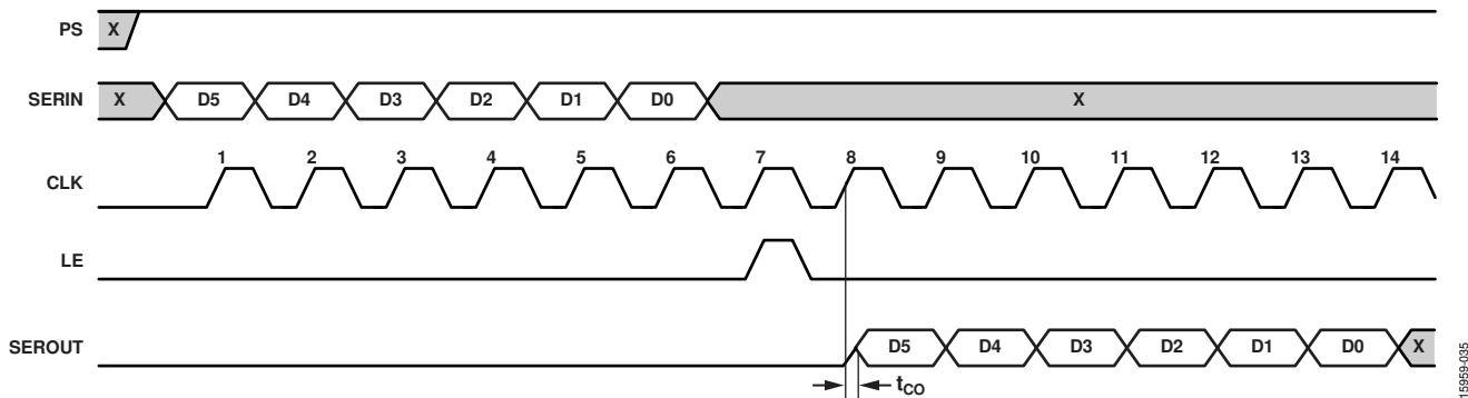
Figure 34. Serial Output Timing Diagram
