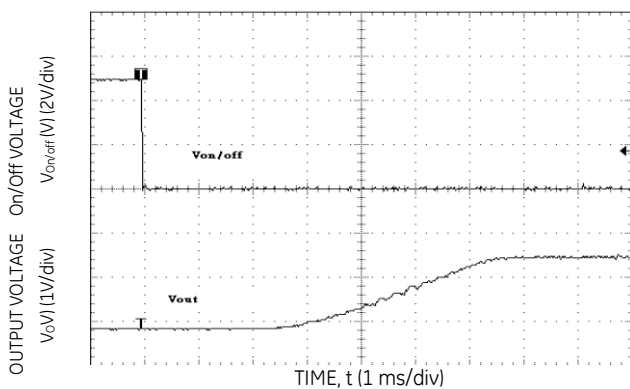
Figure 15. Typical Start-Up Using Remote On/Off with Low-ESR external capacitors ( 7 \times 150\ \mu\text{F} Polymer)
