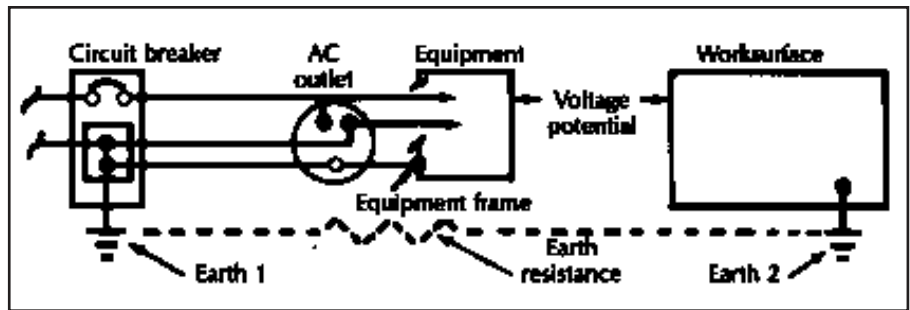
Figure 2. Separate ground systems present potential problems.
