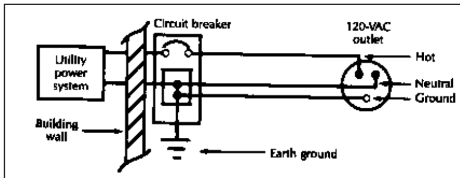
Figure 1. Earth grounding in a typical 120-V, 60-Hz electrical system
