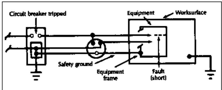
Figure 4. The relationship between equipment (or safety) ground and earth ground.
