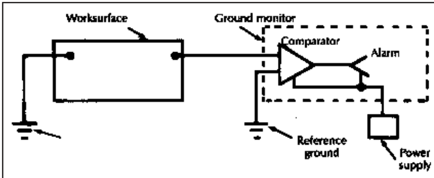
Figure 6. Block diagram of a ground-integrity monitor.
