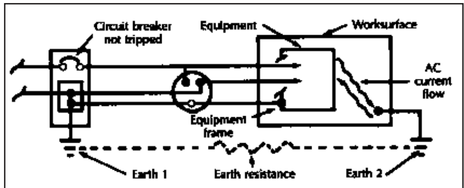
Figure 3. How current flow through a work surface is generated.
