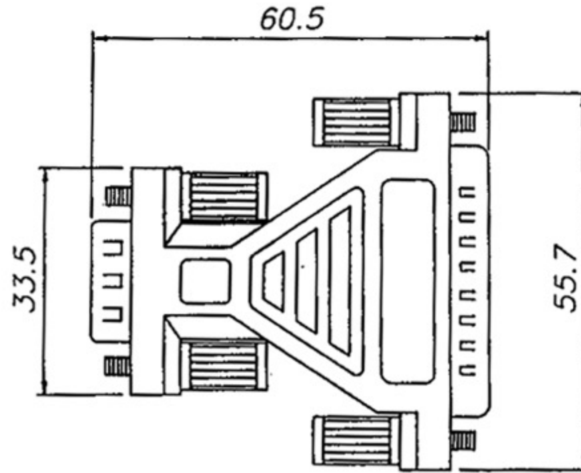
P1 MOLDED
