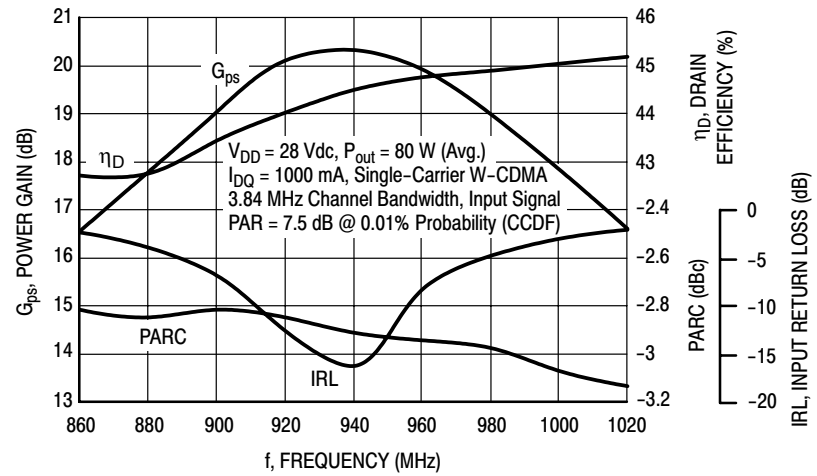
Figure 4. Single-Carrier W-CDMA Broadband Performance @ P out = 80 Watts Avg.
