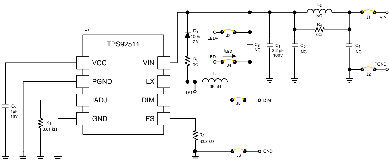
Figure 1. TPS92511EVM Schematic
