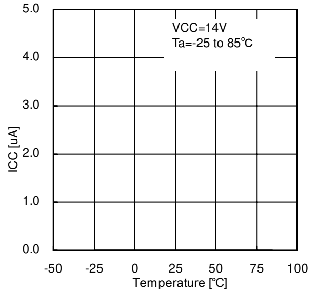
Figure.11 ICC(OFF) - Ta
