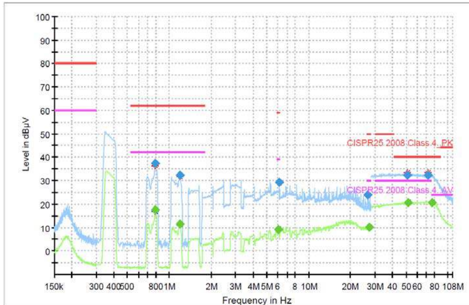
Figure 10 CISPR-25 Class 4 Conducted EMI Scan (Without The Input Common Mode Chock)
