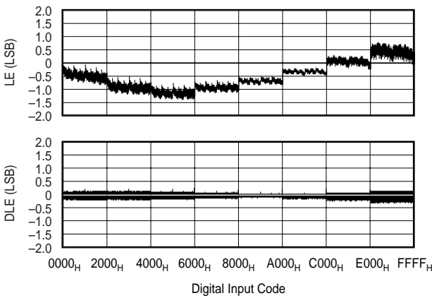
LINEARITY ERROR AND DIFFERENTIAL LINEARITY ERROR vs CODE (DAC C, +25°C)
