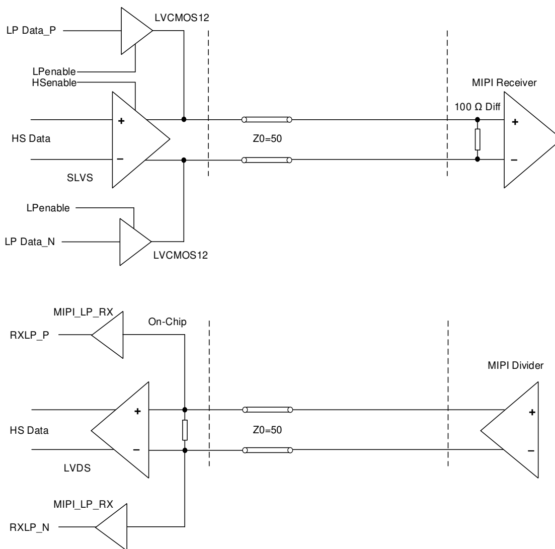
Figure 3.6. MIPI Interface
