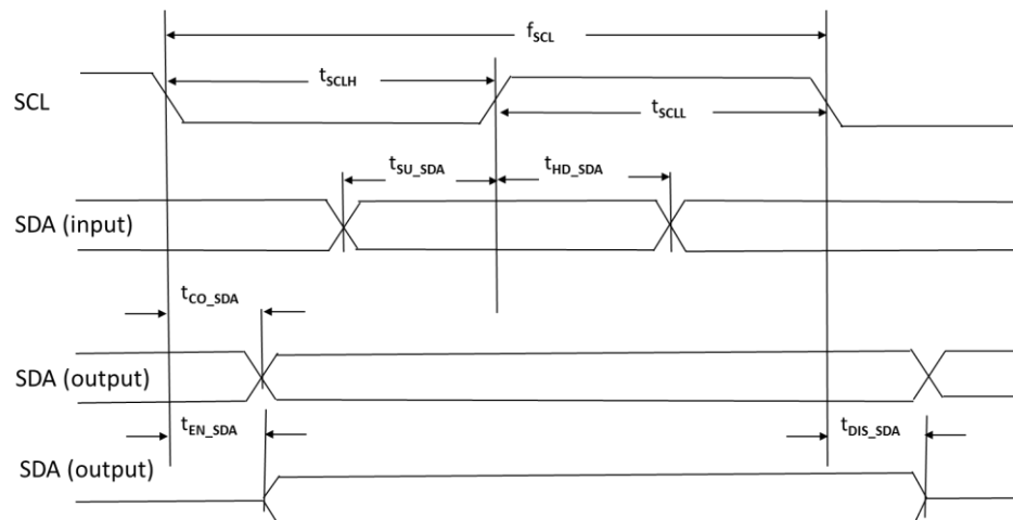
Figure 3.17. I²C /I³C Configuration Timing
