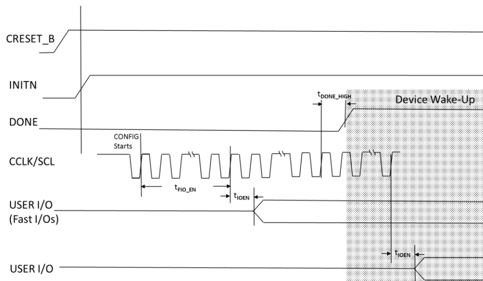
Figure 3.18. Slave SPI/I²C/I³C Wake-Up Timing
