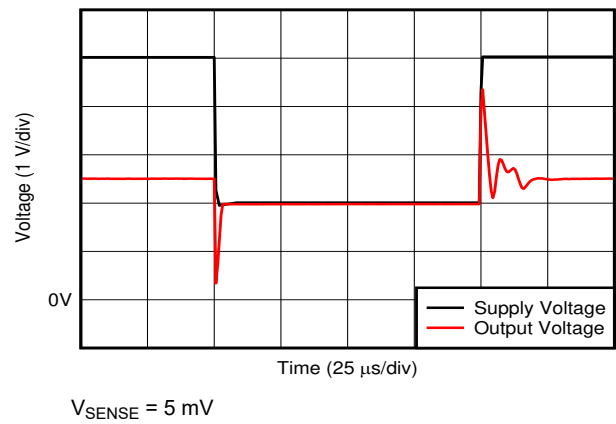
Figure 6-34. Supply Transient Response, A5 Devices
