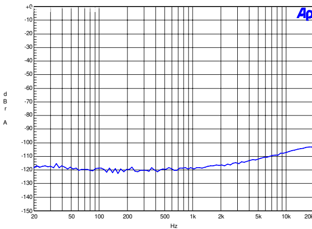
Figure 63. 192 kHz, Crosstalk
