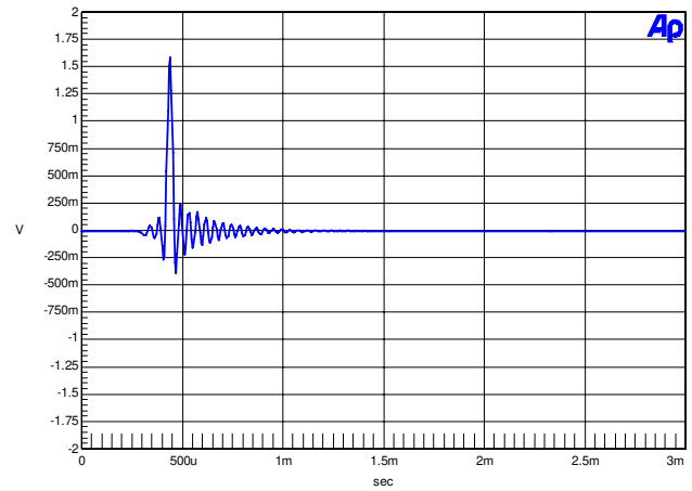
Figure 44. 48 kHz, Impulse Response
