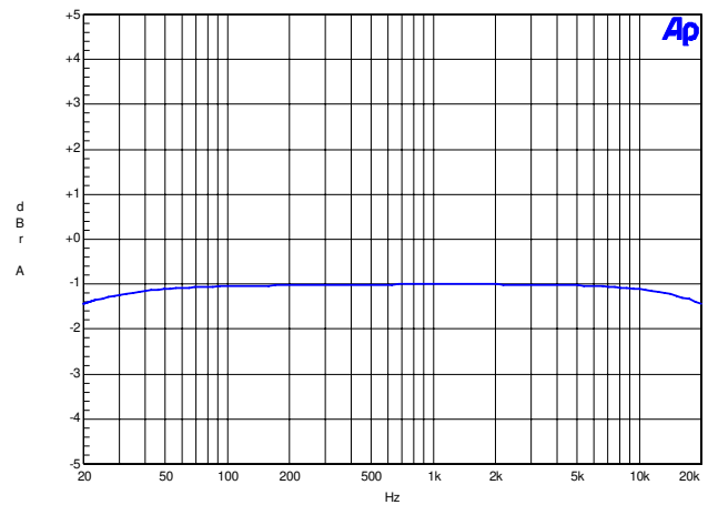
Figure 42. 48 kHz, Frequency Response
