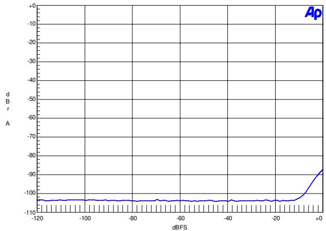
Figure 50. 96 kHz, THD+N vs. Level
