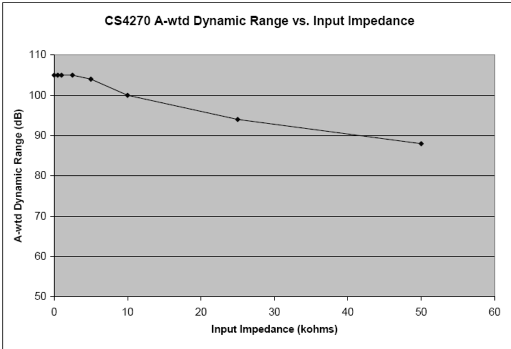
Figure 2. ADC Dynamic Range
