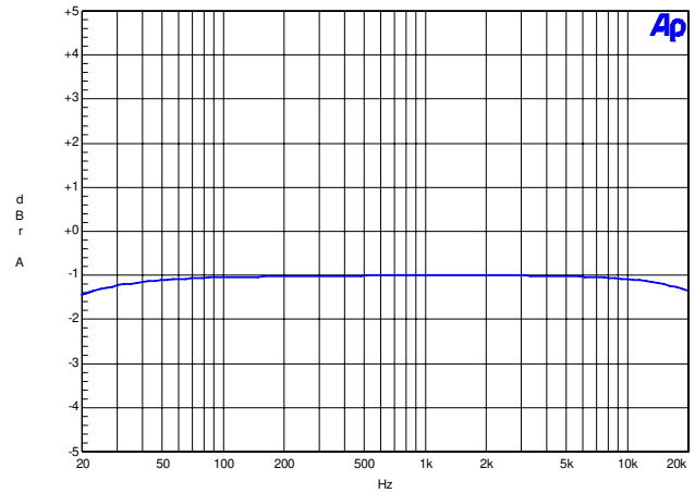
Figure 62. 192 kHz, Frequency Response
