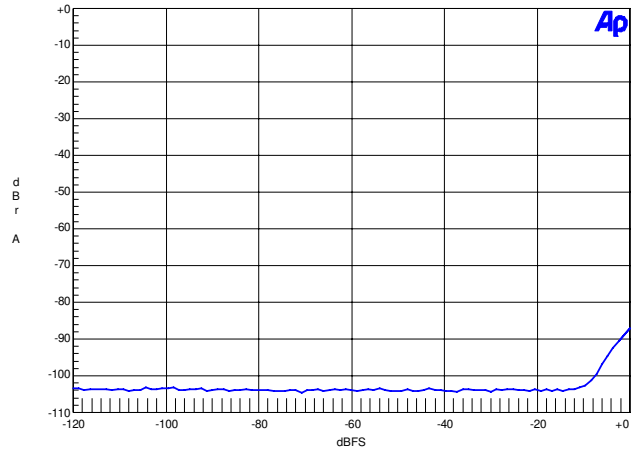
Figure 60. 192 kHz, THD+N vs. Level
