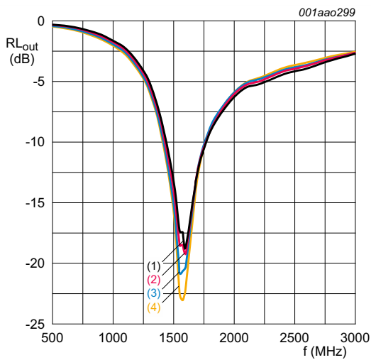
V_{\text{CC}} = 1.8 \text{ V}; P_i = -45 \text{ dBm}. (1) T_{\text{amb}} = -40 \text{ }^\circ\text{C} (2) T_{\text{amb}} = +25 \text{ }^\circ\text{C} (3) T_{\text{amb}} = +85 \text{ }^\circ\text{C} (4) T_{\text{amb}} = +125 \text{ }^\circ\text{C}
