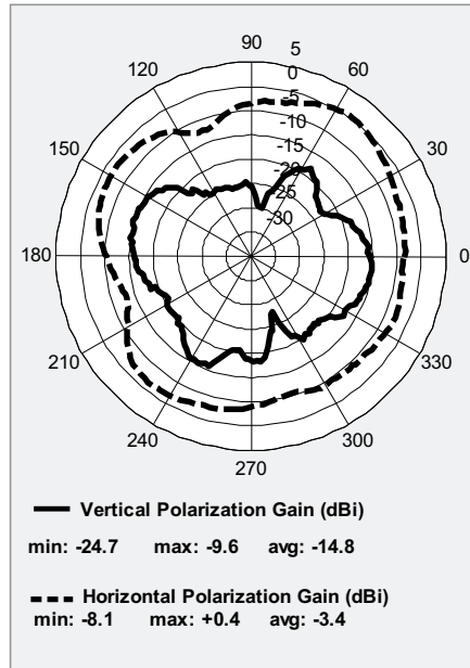
Frequency = 2440 MHz
