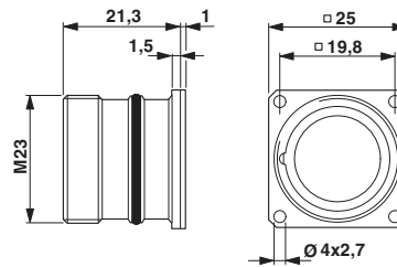
Dimensioned drawing
