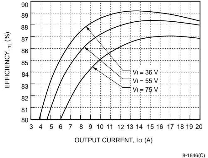
Figure 3. Typical HW100F1 Converter Efficiency vs. Output Current at Room Temperature
