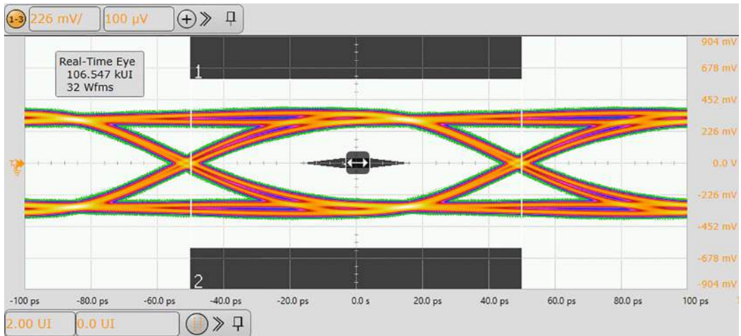
Fig. 6. USB 3.2 eye diagram, PCB with device; typical values
