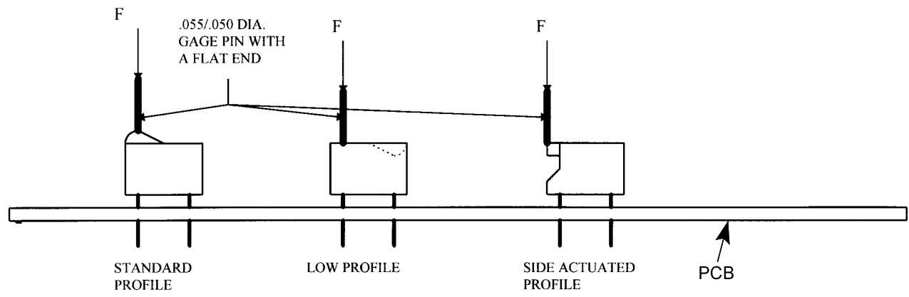
Figure 4 Actuation Force
