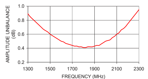
AMPLITUDE UNBALANCE
