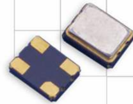
Part Dimensions: 3.2 x 2.5 x 1.0mm • 30.803mg
