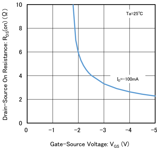
(3) Drain-Source On-State Resistance vs. Gate-Source Voltage
