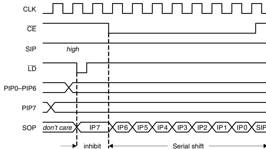
Figure 21. Interface Timing for Parallel-Load and Serial-Shift Operation of the Shift Register
