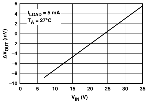
Figure 9. Line Regulation
