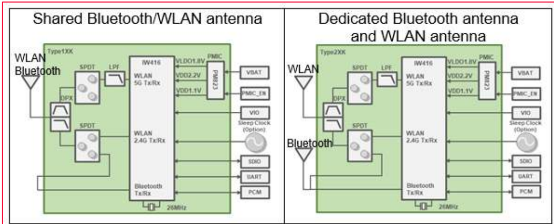
Figure 25: Shared Bluetooth/WLAN Antenna and Dedicated Bluetooth/WLAN Antenna
