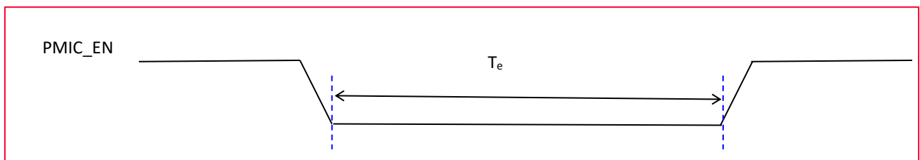
Figure 9: Host Power Off Pin (PMIC_EN) Usage Graph
