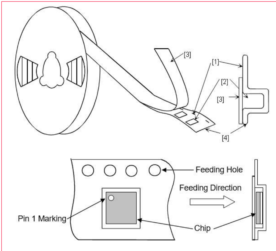
Figure 30: Taping Diagrams
