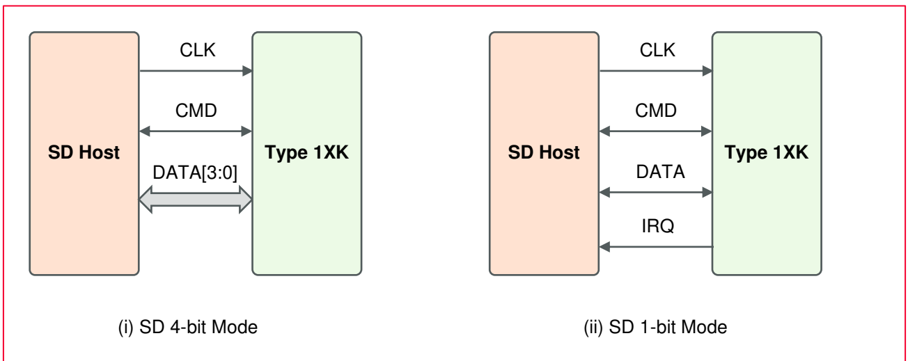
Figure 5: SDIO Pins
