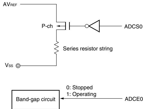
Figure 10-8. How to Reduce Power Consumption in Standby Mode
