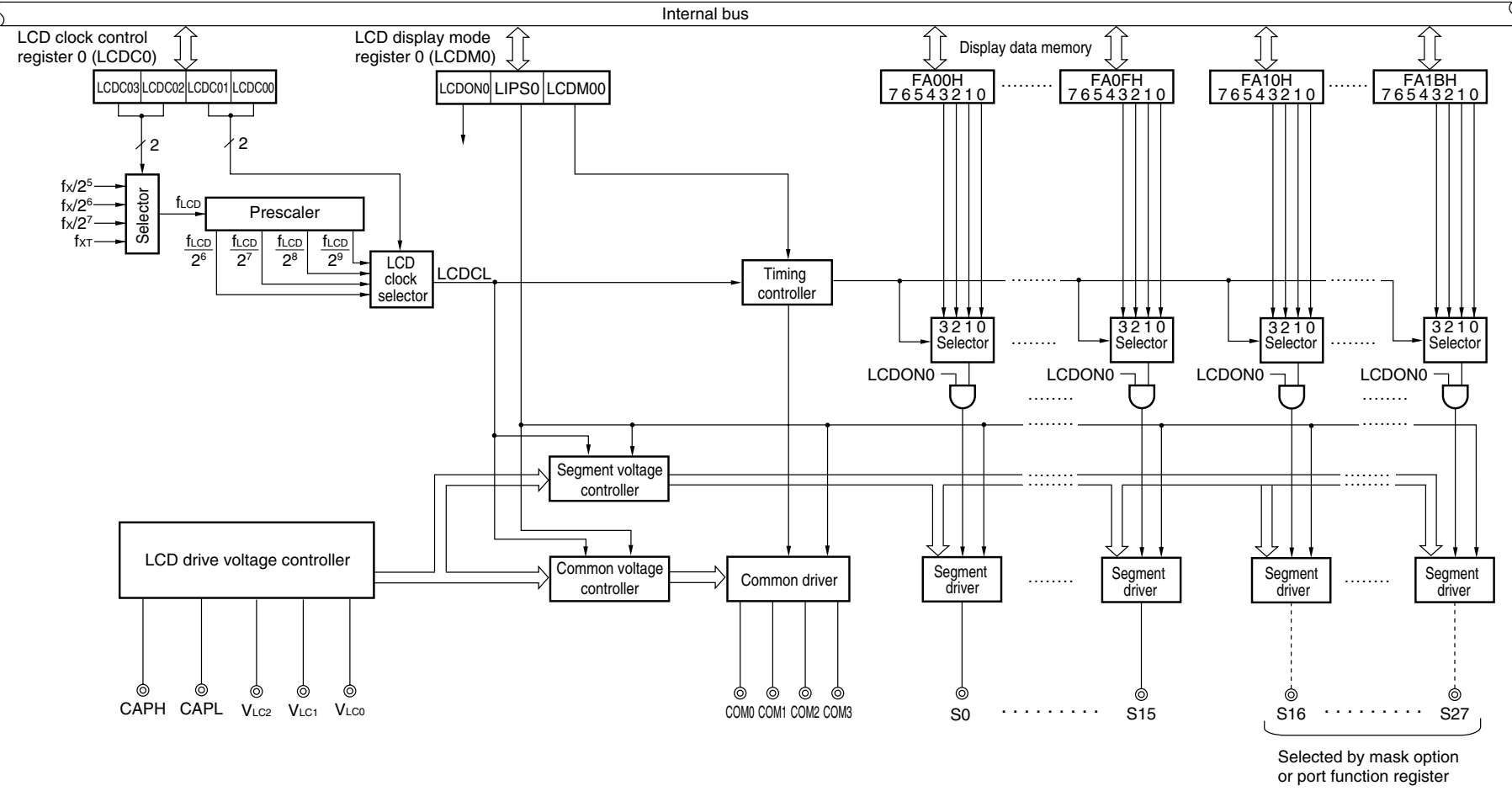
Figure 13-2. LCD Controller/Driver Block Diagram
