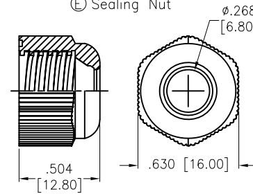
Ⓔ Sealing Nut
