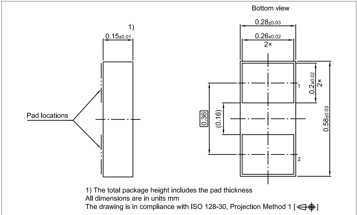
Figure 12 WLL-2-1 package
