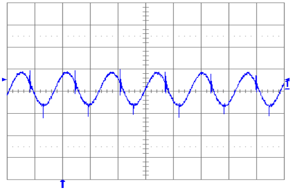
Fig. 3.3V.5: Output voltage ripple ( 20\text{ mV/div.} ) at full rated load current into a resistive load with external capacitance 100\ \mu\text{F} ceramic and V_{in} = 12\text{ V} for V_{out} = 3.3\text{ V} . Time scale: 2\ \mu\text{s/div.}
