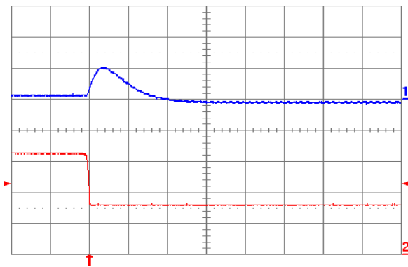
Fig. 1.0V.7: Output voltage response for V_{out} = 1.0\text{ V} to negative load current step change from 16\text{ A} to 8\text{ A} with slew rate of -5\text{ A}/\mu\text{s} at V_{in} = 12\text{ V} . Top trace: output voltage ( 200\text{ mV/div.} ); Bottom trace: load current ( 5\text{ A/div.} ). C_o = 100\ \mu\text{F} ceramic. Time scale: 20\ \mu\text{s/div.}
