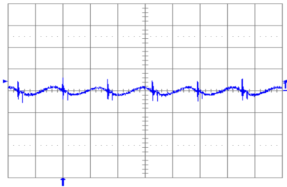
Fig. 1.0V.5: Output voltage ripple ( 20\text{ mV/div.} ) at full rated load current into a resistive load with external capacitance 100\ \mu\text{F} ceramic and V_{in} = 12\text{ V} for V_{out} = 1.0\text{ V} . Time scale: 2\ \mu\text{s/div.}
