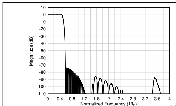
Figure 7-29. Linear Phase Decimation Filter Magnitude Response
