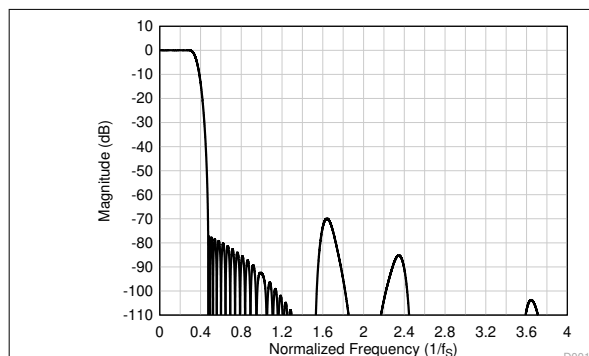
Figure 7-31. Linear Phase Decimation Filter Magnitude Response
