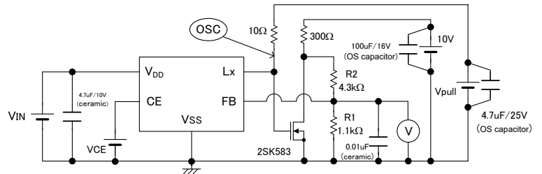
Circuit ④
