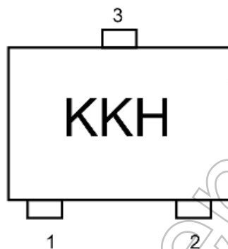
Fig. 6.1 Marking
