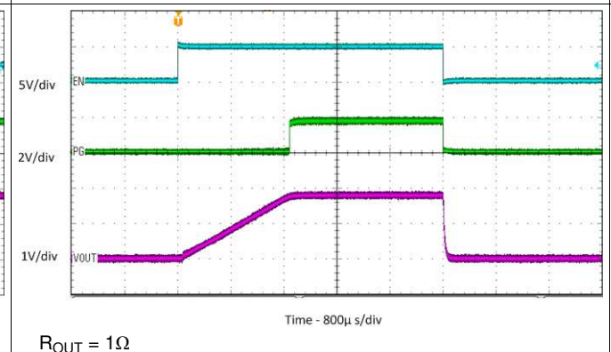
Figure 29. Startup / Shutdown with Resistance Load
