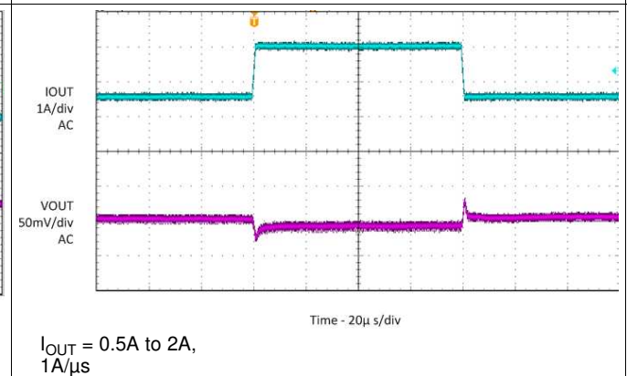
Figure 27. Load Transient
