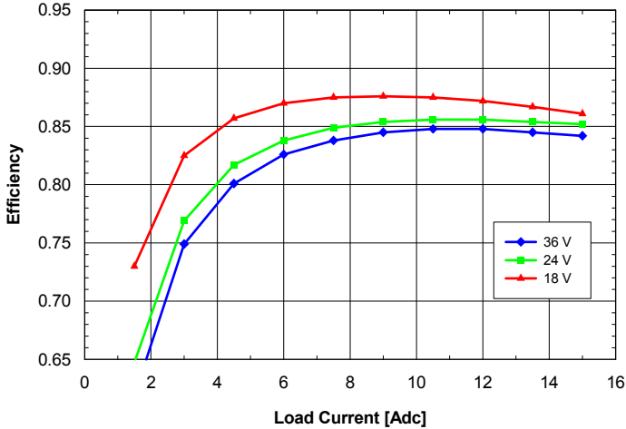
Fig. 2.0V.5: Efficiency vs. load current and input voltage for SQ24T/S15020 converter mounted vertically with air flowing from pin 3 to pin 1 at a rate of 300 LFM (1.5 m/s) and T_a = 25^\circ\text{C} .
