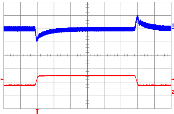
Fig. 1.2V.11: Output voltage response to load current step-change (3.75 A – 7.5 A – 3.75 A) at V_{in} = 24V . Top trace: output voltage (100 mV/div.). Bottom trace: load current (5 A/div.). Current slew rate: 0.1 A/ \mu s . C_o = 1 \mu F ceramic. Time scale: 0.2 ms/div.
