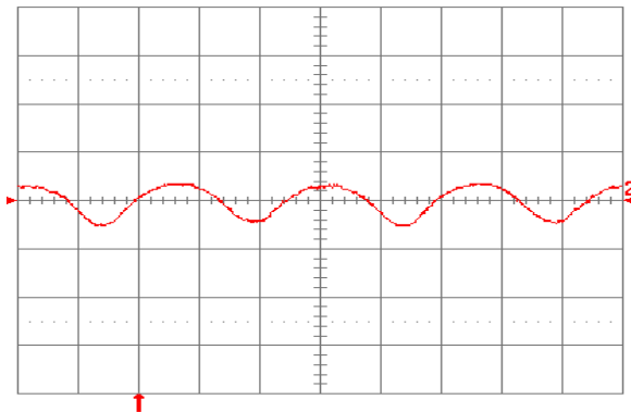
Fig. 1.2V.15: Input reflected ripple current, i_c (100 mA/div.), measured at input terminals at full rated load current and V_{in} = 24\text{V} . Refer to Fig. 1.2V.14 for test setup. Time scale: 1 \mu\text{s}/\text{div} .
