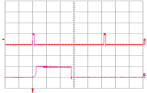
Fig. 3.3V.18: Load current (top trace, 20 A/div., 20 ms/div.) into a 10 mΩ short circuit during restart, at V in = 24V. Bottom trace (20 A/div., 1 ms/div.) is an expansion of the on-time portion of the top trace.
