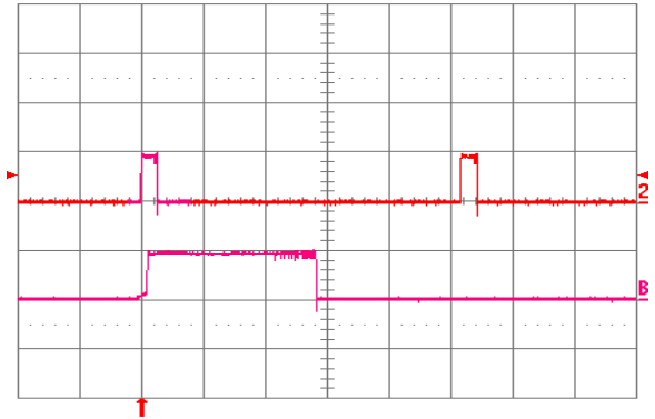
Fig. 2.0V.18: Load current (top trace, 20 A/div., 20 ms/div.) into a 10 mΩ short circuit during restart, at V in = 24V. Bottom trace (20 A/div., 2 ms/div.) is an expansion of the on-time portion of the top trace.
