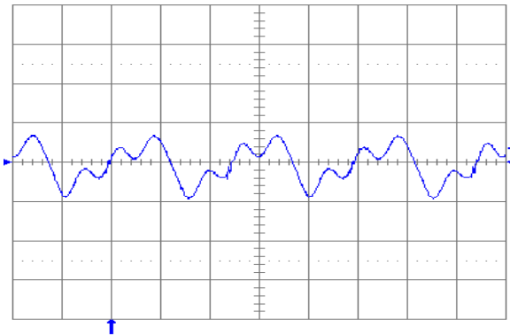
Fig. 2.0V.13: Output voltage ripple (20 mV/div.) at full rated load current into a resistive load with C_o = 10 \mu\text{F} tantalum + 1\mu\text{F} ceramic and V_{in} = 24 \text{ V} . Time scale: 1 \mu\text{s}/\text{div} .
