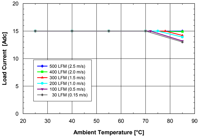
Fig. 2.0V.1: Available load current vs. ambient air temperature and airflow rates for SQ24T15020 converter with B height pins mounted vertically with V_{in} = 24V , air flowing from pin 3 to pin 1 and maximum FET temperature \leq 120^{\circ}C .
