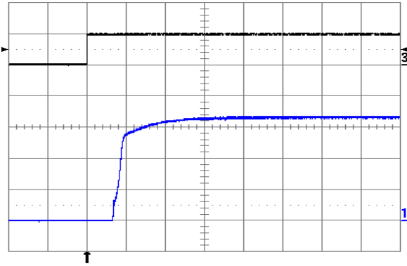
Fig. 3.3V.9: Turn-on transient at full rated load current (resistive) with no output capacitor at V_{in} = 24V , triggered via ON/OFF pin. Top trace: ON/OFF signal (5 V/div.). Bottom trace: output voltage (1 V/div.). Time scale: 2 ms/div.
