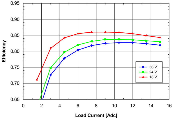
Fig. 1.5V.5: Efficiency vs. load current and input voltage for SQ24T/S15015 converter mounted vertically with air flowing from pin 3 to pin 1 at a rate of 300 LFM (1.5 m/s) and T_a = 25^\circ\text{C} .
