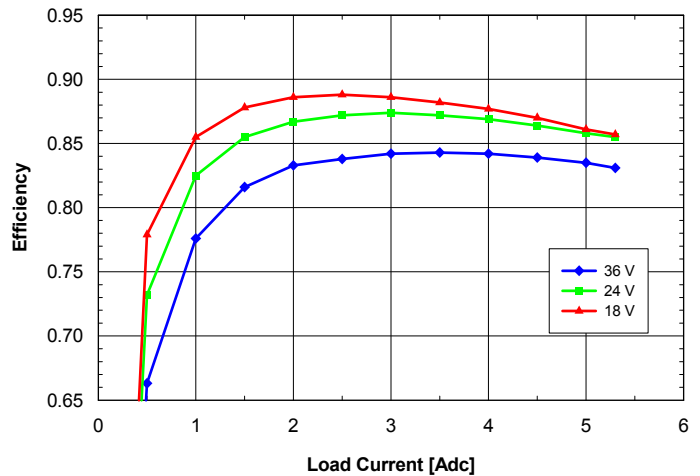
Fig. 8.0V.2: Efficiency vs. load current and input voltage for SQ24T/S05080 converter mounted vertically with air flowing from pin 3 to pin 1 at a rate of 300 LFM (1.5 m/s) and T_a = 25\text{ }^\circ\text{C} .
