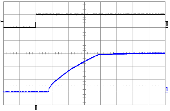
Fig. 6.0V.10: Turn-on transient at full rated load current (resistive) plus 10,000 \mu F at V_{in} = 24V , triggered via ON/OFF pin. Top trace: ON/OFF signal (5 V/div.). Bottom trace: output voltage (2 V/div.). Time scale: 2 ms/div.
