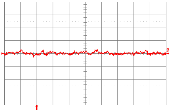
Fig. 1.2V.16: Input reflected ripple current, i_s (10 mA/div.), measured through 10 \mu\text{H} at the source at full rated load current and V_{in} = 24\text{V} . Refer to Fig. 1.2V.14 for test setup. Time scale: 1 \mu\text{s}/\text{div} .
