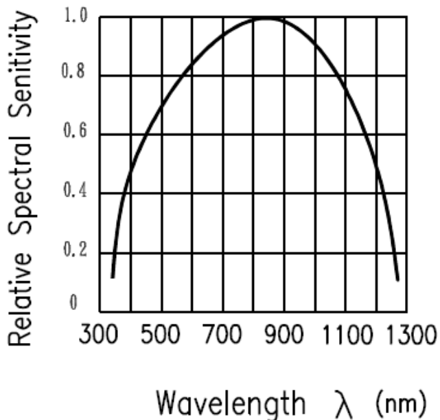
Spectral Sensitivity
