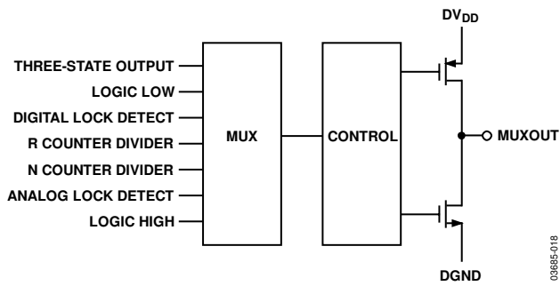
Figure 16. MUXOUT Schematic
