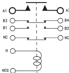
Circuit Configuration 10
