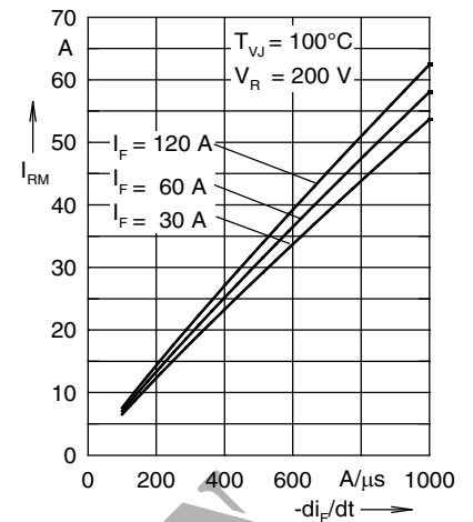
Fig. 3 Typ. peak reverse current I_{RM}
