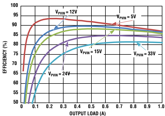
FIGURE 10. EFFICIENCY vs LOAD, PWM, V_{OUT} = 3.3V
