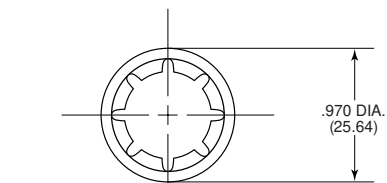
55-025B INTERNAL TOOTH PUSH-ON LOCKWASHER For panels greater than .105" (2.67) thickness
